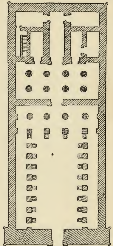
FIG. 37. GROUND-PLAN OF THE TEMPLE OF RAMSES III. KARNAK.
